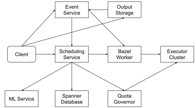
Figure 3: Build service architecture
